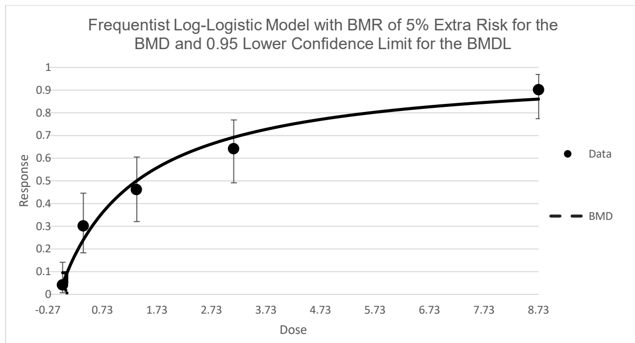
Figure A3.3 Log-logistic model output for increased histiocytic infiltration of the liver in female mice (NTP, 2008)
